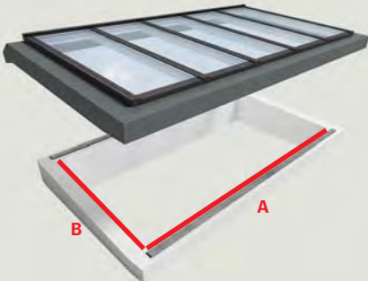
Sub-construction A: Opening Width B: Opening Length
